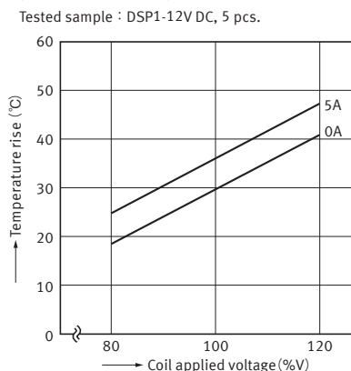
3.-(2) Coil temperature rise (1 Form A 1 Form B)
