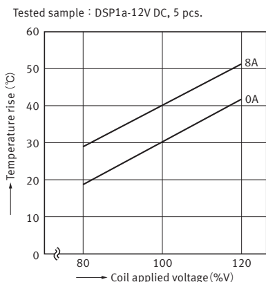
3.-(1) Coil temperature rise (1 Form A)
