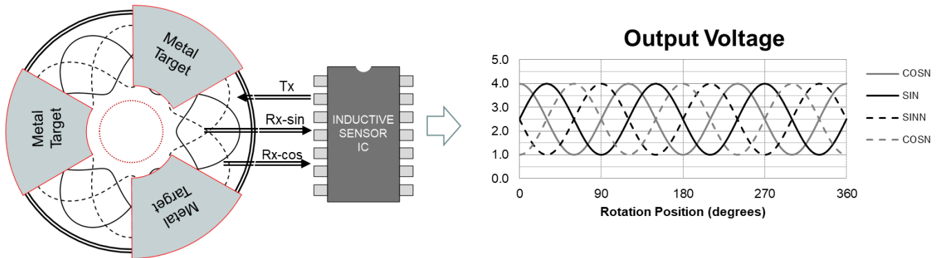
Figure 28. Coil Design and Signal Output for a 3 × 120° Rotary Sensor
