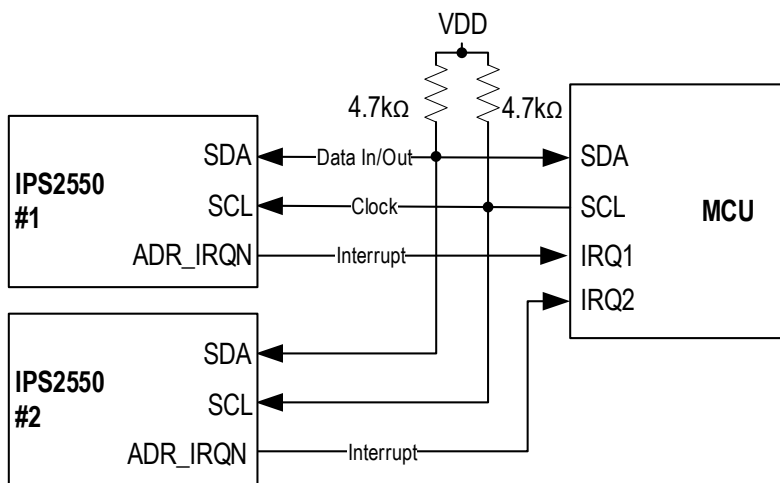
Figure 18. I2C Interface Configuration with Multi-slave Interrupt
