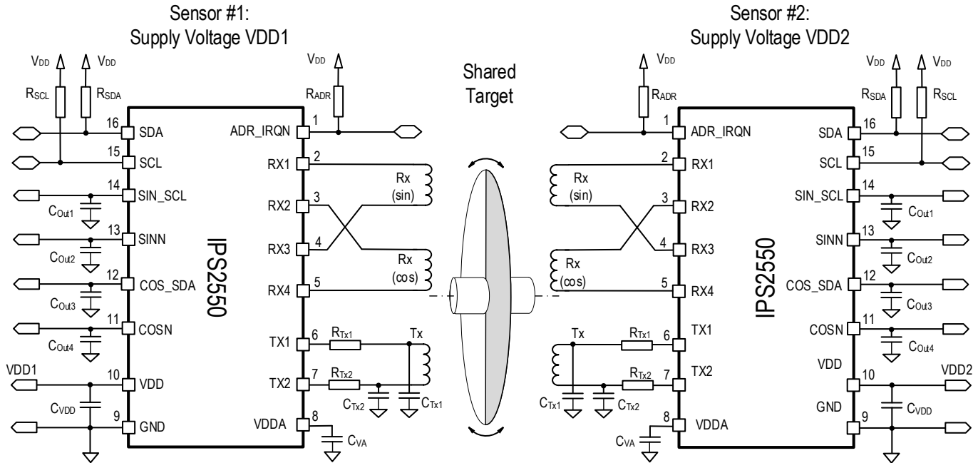
Figure 25. Application Diagram: Dual Redundant Sensors, Dual Supply
