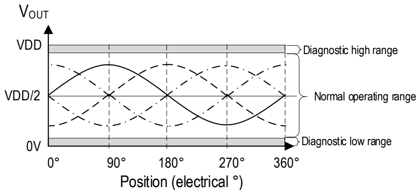
Figure 21. Operating Range and Diagnostic Range
