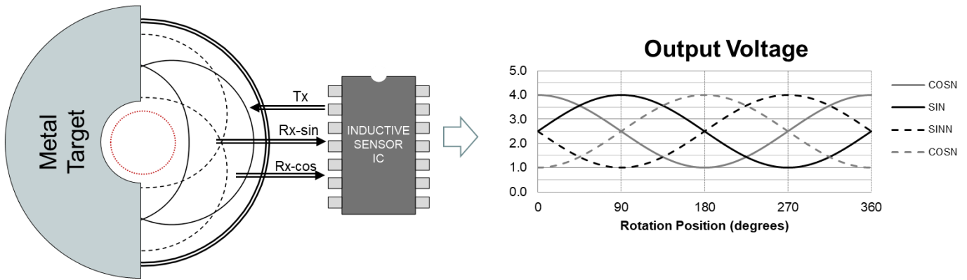
Figure 26. Coil Design and Signal Output for a 360° Rotary Sensor
