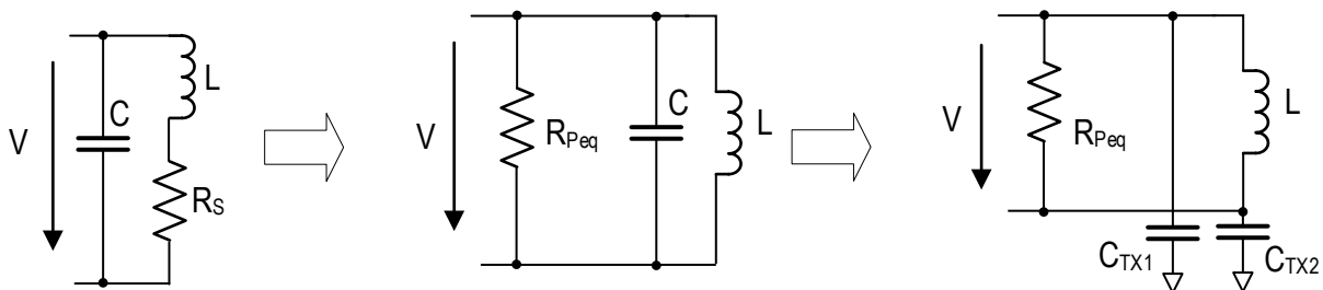
Figure 5. Parallel Resonator Circuit
