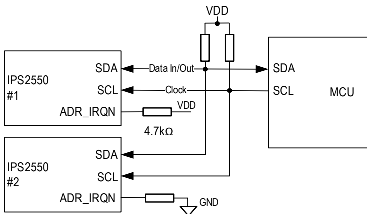
Figure 15. I2C Interface with Address Select
