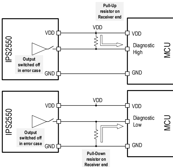
Figure 22. Selection of Diagnostic Range
