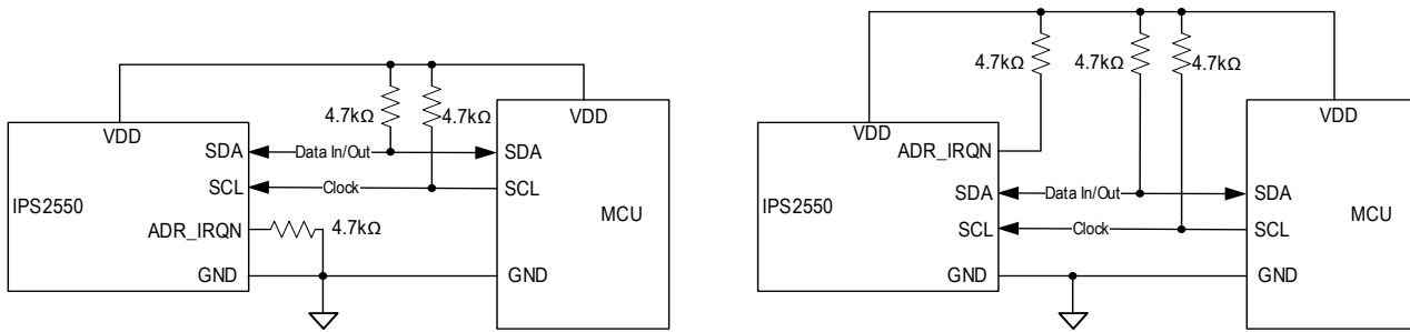
Figure 16. I2C Interface with Address Selection by Hardware Pin Strapping Through ADR_IRQN Pin
