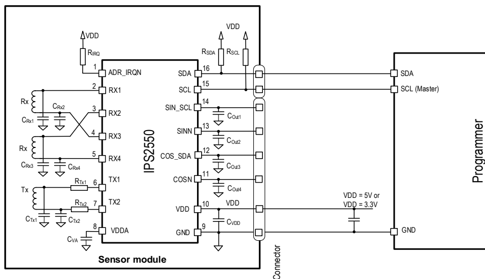
Figure 19. Programming the IPS2550 over the I2C Interface
