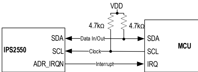
Figure 17. I2C Interface Configuration with Interrupt on a Single Slave
