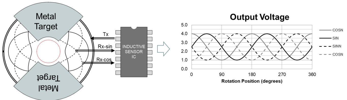
Figure 27. Coil Design and Signal Output for a 2 × 180° Rotary Sensor
