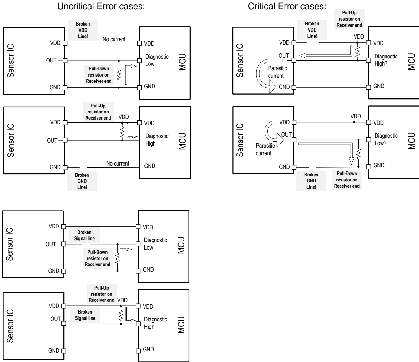
Figure 23. Parasitic currents with Broken VDD or Broken GND lines
