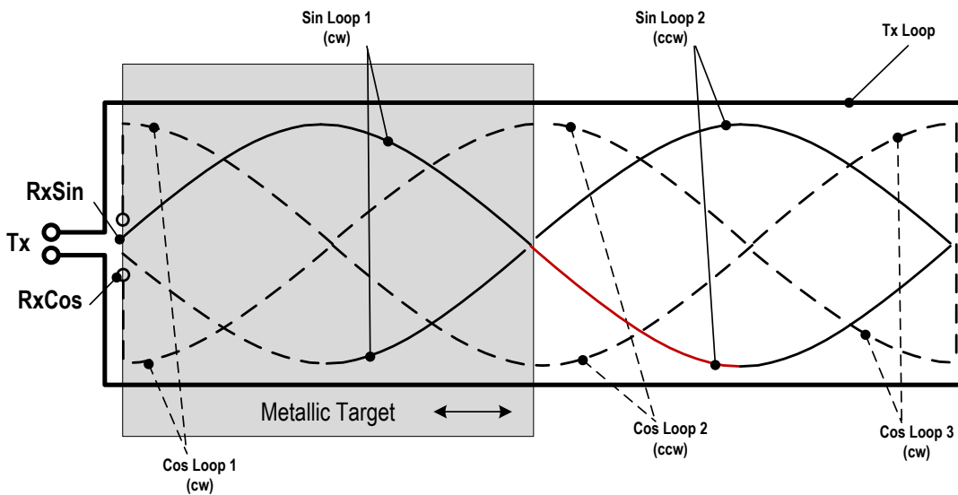
Figure 7. Coil Design for a Linear Motion Sensor
