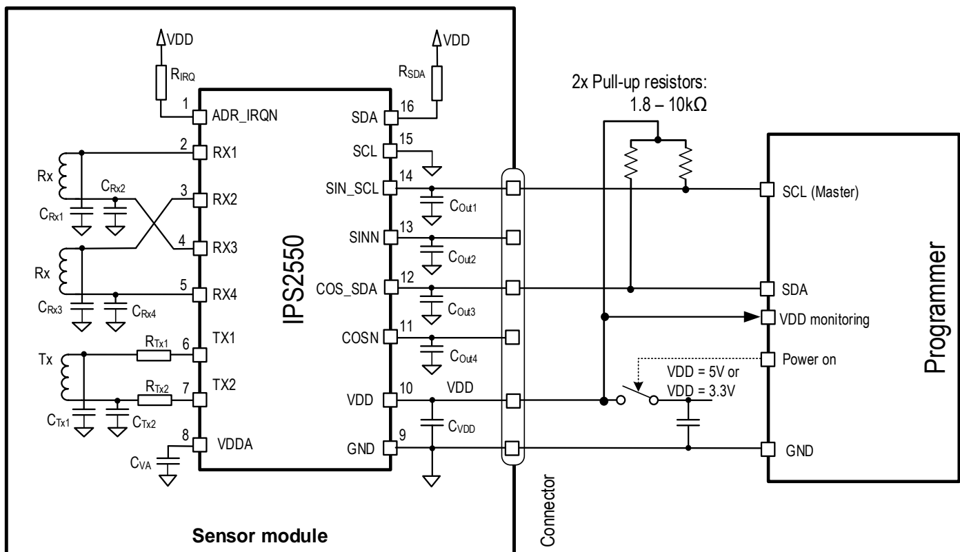
Figure 20. End of Line Programming of the IPS2550 Through the Analog Outputs
