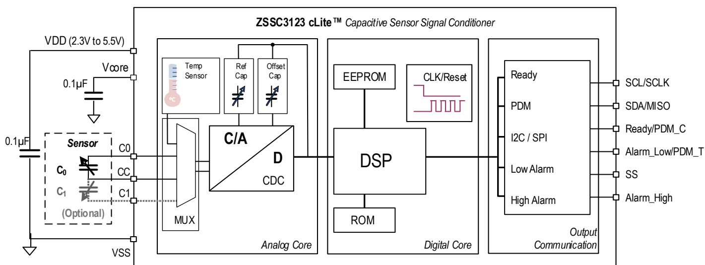
Figure 9. ZSSC3123 Block Diagram
